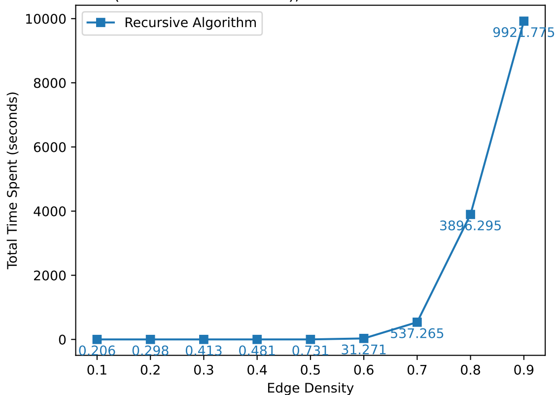
Overall Time Spent on Recursive Algorithm at Different Edge Densities (200 realizations each), basis calculation disabled
